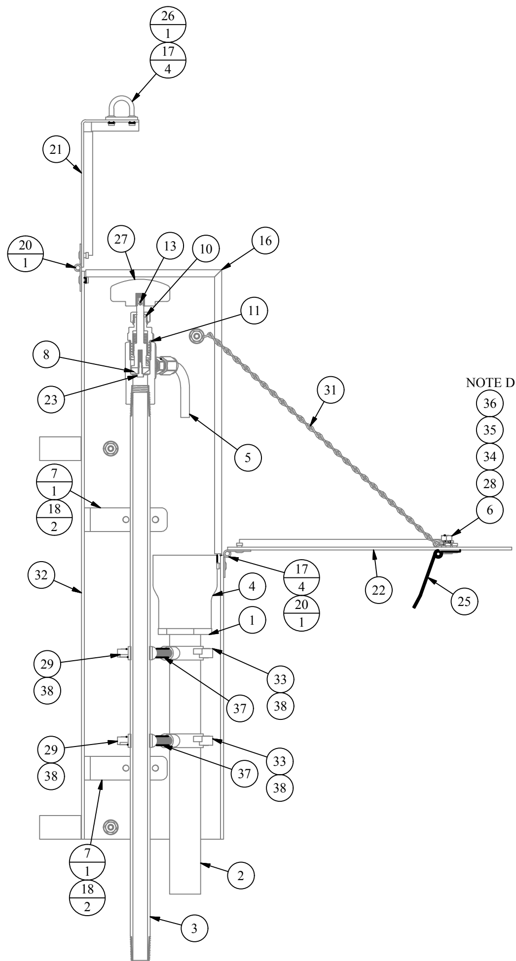
SECTION A-A CENTER SECTION VIEW
