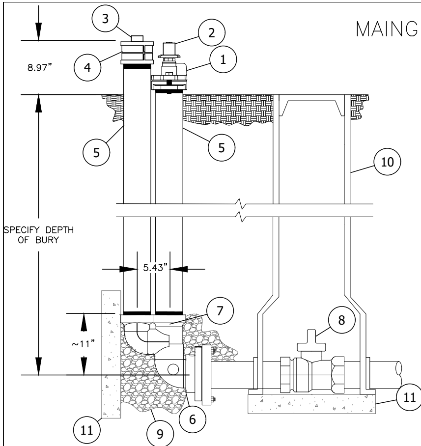
1 SIDE VIEW Scale: 3/4"=1'-0"
