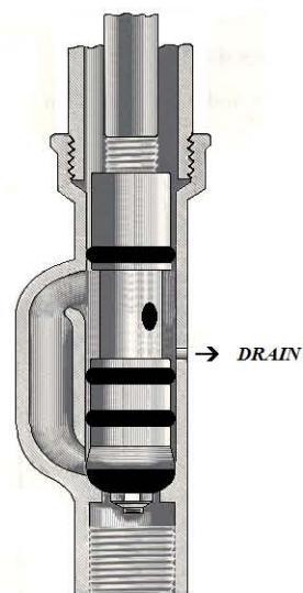
COMPRESSION TYPE HYDRANT
