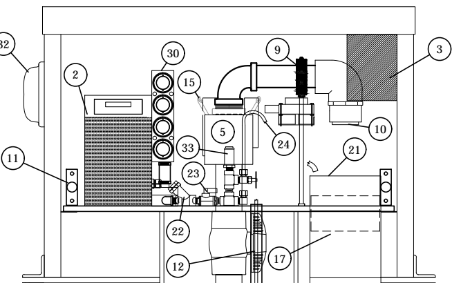
B ENCLOSURE - CUT VIEW (FRONT)
