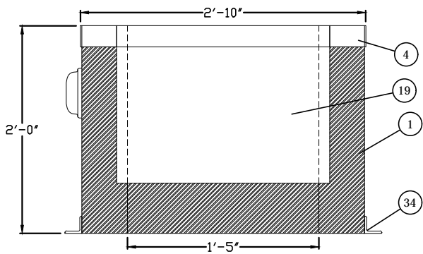
A ENCLOSURE - CLOSED (FRONT)
